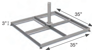
Steel Base 35" x 35"
